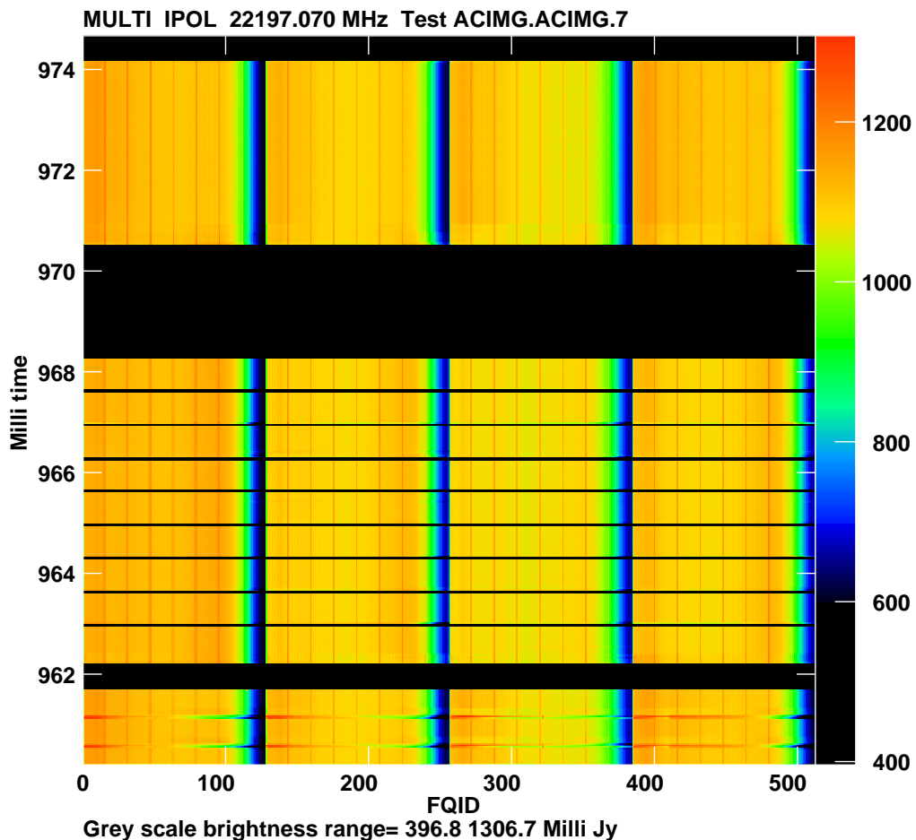
Example of output from ACIMG. The x axis is FQID (frequency ID number) because the channel increments over all 4 spectral windows is not entirely regular. The time axis is labeled in days.
